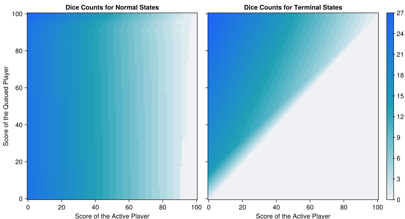
Figure 2 | Optimal rolls for each state given the standard ruleset of M = 100, s = 6 . For normal states, there is a weak correlation between the opponents score and the optimal number of dice to throw. For terminal states, the optimal policy while ahead is to stand . For terminal states where victory is not guaranteed, there is a positive correlation between the difference in the queued score and the active score, and the optimal number of dice to roll. This accounts for the diagonal bands.
