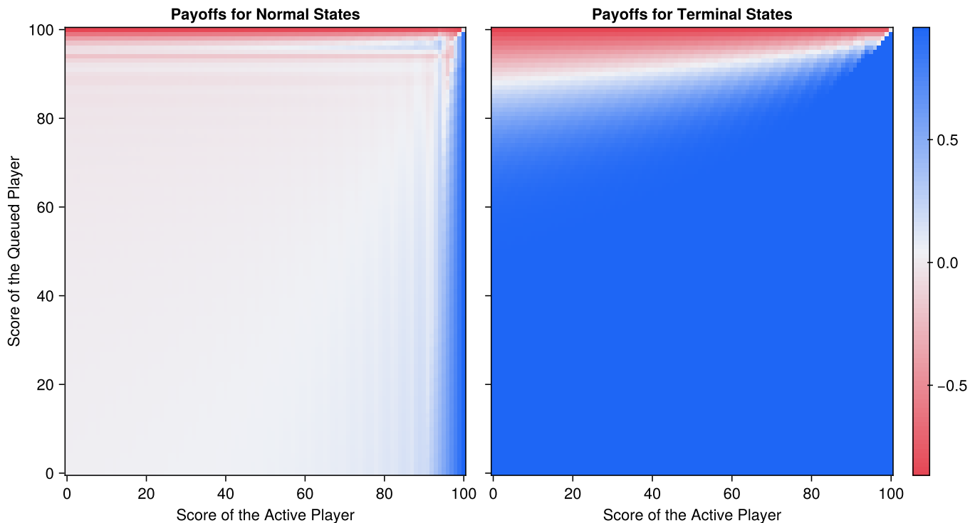
Figure 1 | Optimal payoffs for each state given the standard ruleset of M = 100, s = 6 . In terminal states, there is a logarithmic curve which marks where the odds are equal. For normal states, there are distinct bands spaced s apart in which the payoffs are more in favor of the player who is ahead. There is also the inverse icicles , which are the little bands near (M, M) where the advantage switches to the player who is behind.
